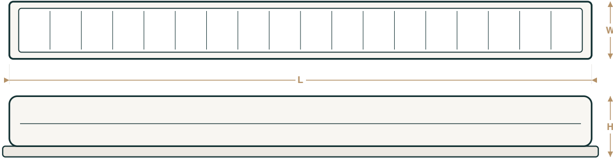
SIDE ELEVATION
