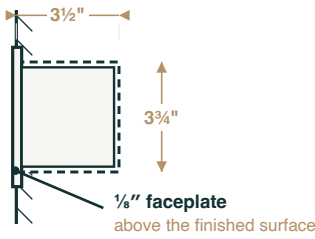
SIDE — masonry box by others 3 3/4" x 3 1/2" x 11" masonry box, 6 gang (RACO TP965 or equal)
