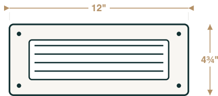
LOUVERED FACE (LV) — brushed stainless nickel louwer assembles over the standard trim plate · 3/8" above the surface
