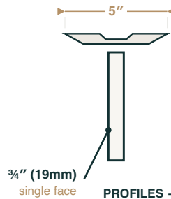
PROFILES — CANOPY PLATE · FACE DEPTHS
