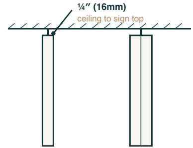
TOP — SINGLE · DOUBLE FACE universal bracket — end / top mount
