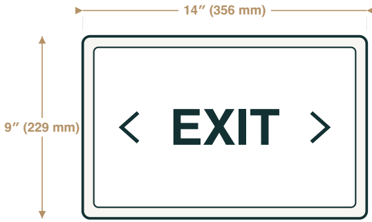
FRONT — STANDARD MOUNTS universal field-adjustable chevron arrows
