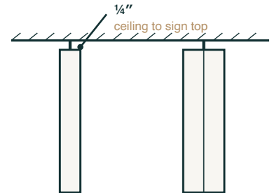
TOP — SINGLE · DOUBLE FACE universal bracket — end / top mount
