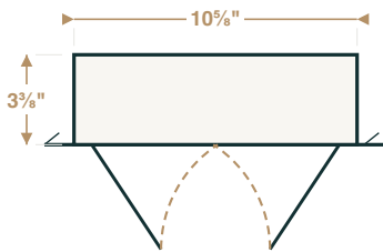
TOP VIEW — doors adjustable through 90°, emergency mode
