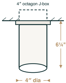
STANDARD TOP MOUNT canopy plate over the J-box
